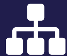
BPM & Workflow
